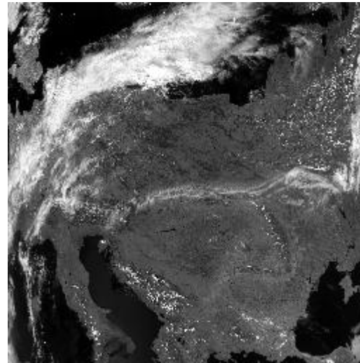
AVHRR: Channel #2
