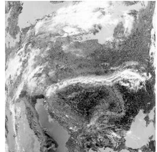
AVHRR: Channel #3
