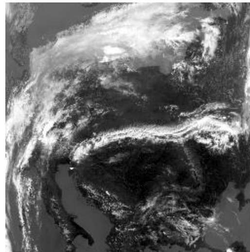
AVHRR: Channel #4
