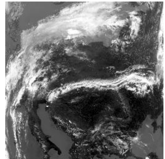
AVHRR: Channel #5
