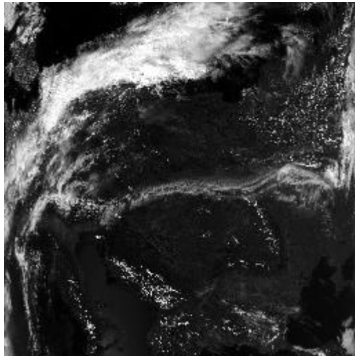
AVHRR: Channel #1
